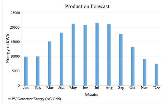
Fig 3. Monthly energy production forecasts when the tilt angle of the photovoltaic panels is 32°
