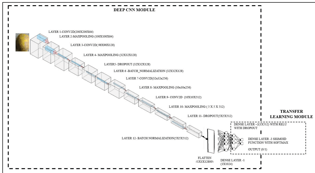
Fig 2. Proposed Architecture
