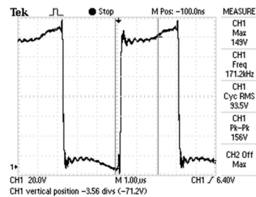
Fig. 8. Voltage on transistor VT3
