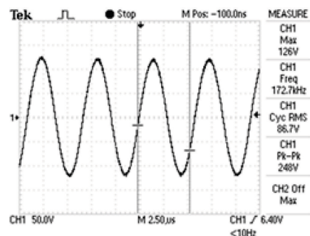
Fig. 2. Oscilloscope of voltage UC4
